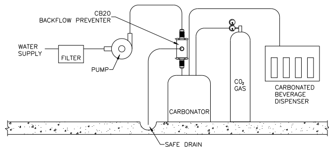
CARBONATED BEVERAGE SYSTEM
