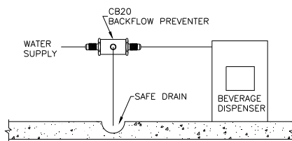
NON-CARBONATED BEVERAGE SYSTEM
