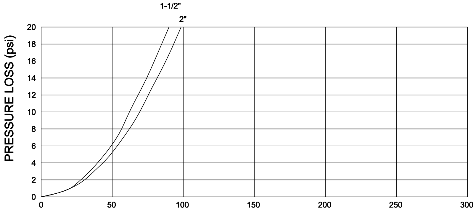
FLOW RATE (gpm) VALVE TESTED FULLY OPEN WITH NO SPRING
